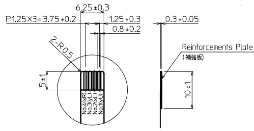
DETAIL C (2:1)
