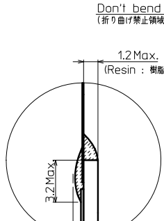
DETAIL D (5:1)
